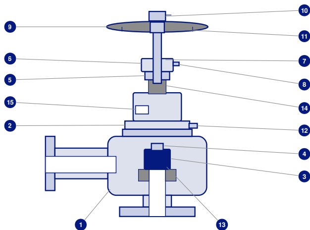
FIG. 2 | SECTIONAL ARRANGEMENT
