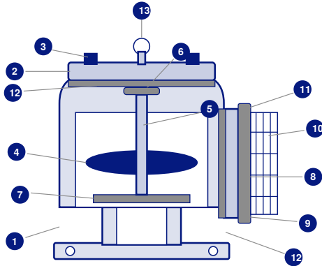
FIG. 2 | SECTIONAL ARRANGEMENT
