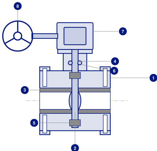
FIG. 2 | SECTIONAL ARRANGEMENT
