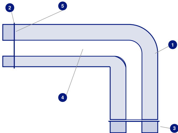
FIG. 2 | ELBOW 90°, SECTIONAL ARRANGEMENT
