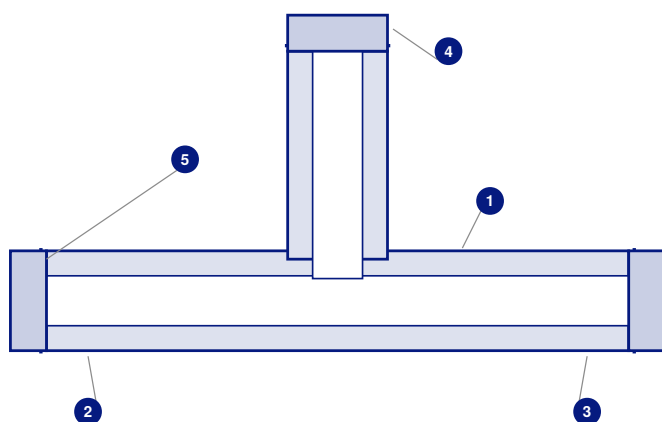
FIG. 2 | EQUAL TEE, SECTIONAL ARRANGEMENT
