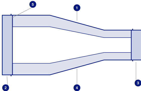
FIG. 2 | CONCENTRIC REDUCER, SECTIONAL ARRANGEMENT
