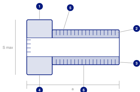
FIG. 2 | SECTIONAL ARRANGEMENT
