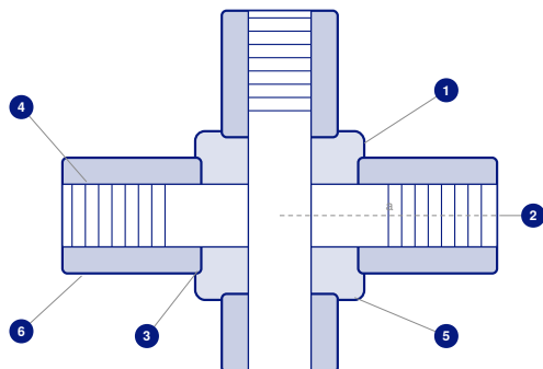
FIG. 2 | SECTIONAL ARRANGEMENT
