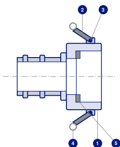
FIG. 2 | SECTIONAL ARRANGEMENT, SCHEMATIC
