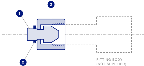
FIG. 2 | SECTIONAL ARRANGEMENT ON FITTING PORT
