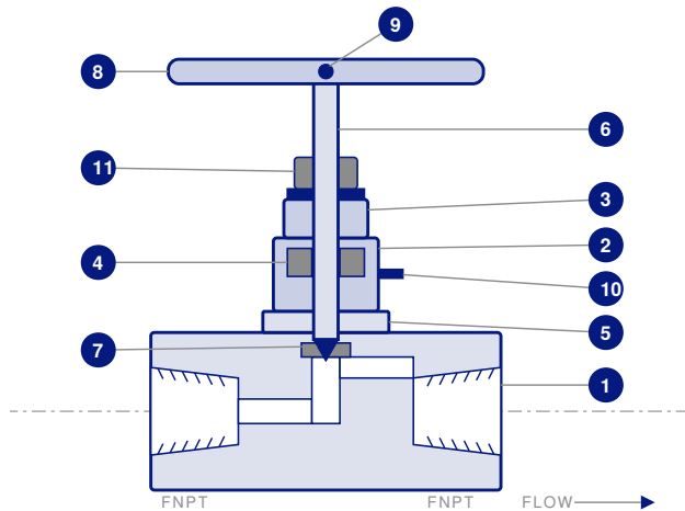
FIG. 2 | SECTIONAL ARRANGEMENT
